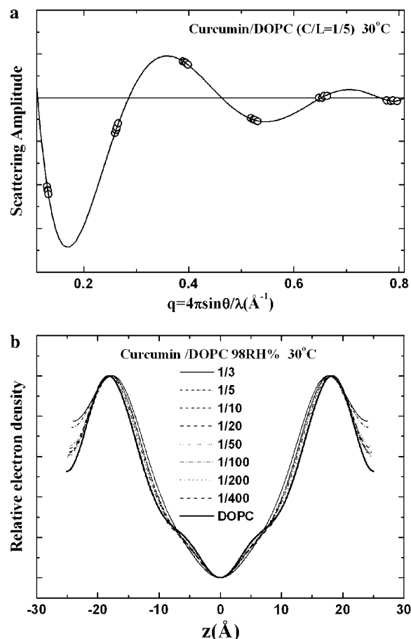
FIGURE 5 ( a ) An example of a phasing diagram for DOPC bilayers containing curcumin at C_b/L = 1:5 by the swelling method (23). Several sets of data points were obtained from diffraction measured at different humidity levels to change the lamellar spacing. One set of data was used to construct the Shannon curve (solid line). The phases (i.e., the signs of the amplitudes) were chosen such that the curve would go through all the data points. ( b ) With the phases determined, the diffraction amplitudes were used to construct the electron density profiles for DOPC bilayers containing curcumin at different C_b/L , all at 30°C and 98% RH.
