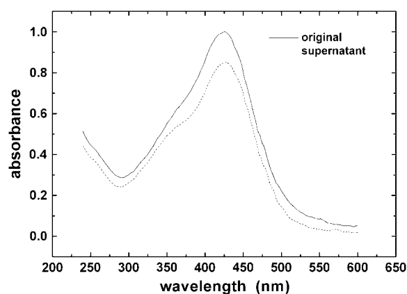
FIGURE 1 Absorption spectrum of curcumin in the original 25 \mu\text{M} solution (solid line) and in the supernate after centrifugation (dotted line). The background absorption by the buffer has been removed. Taking into account the curcumin loss to the wall of the centrifuge tube ( \sim 10\% ), the spectral amplitude of the supernate at 426 nm was estimated to be 97% of the original solution before centrifugation.
